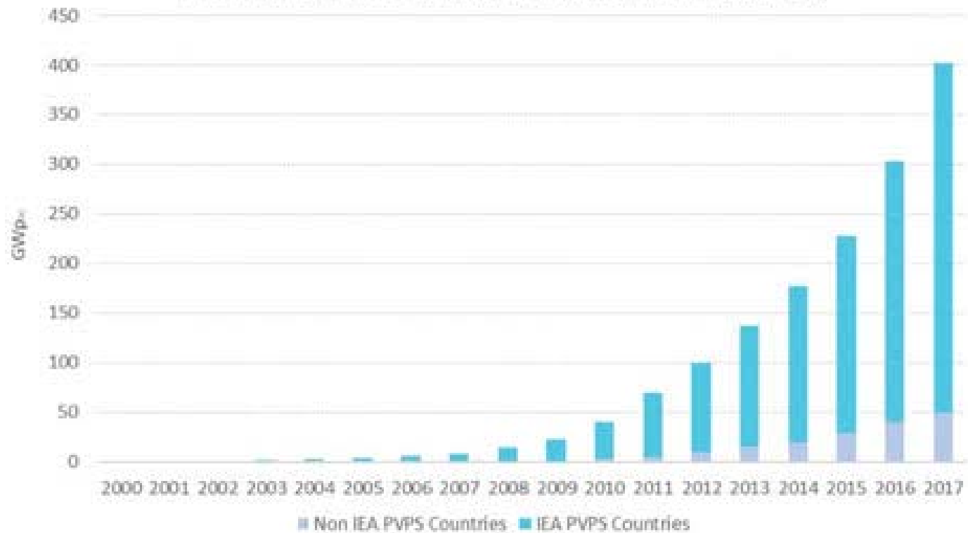
FIGURE 2: EVOLUTION OF TOTAL INSTALLED CAPACITY (GW - DC)
